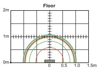
Luminous flux emergency / mains: 90lm
