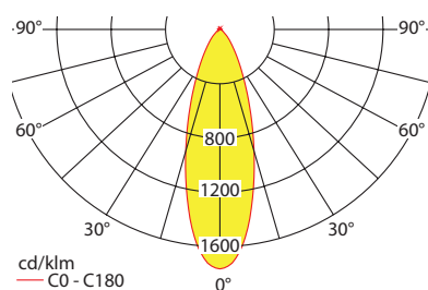
Luminous flux emergency / mains: 90lm
