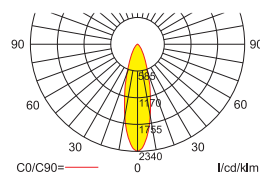
Luminous flux: 280 lm
