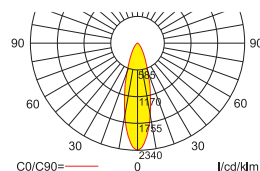
Luminous flux: 120 lm
