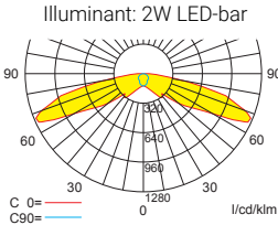
Ceiling mounting
