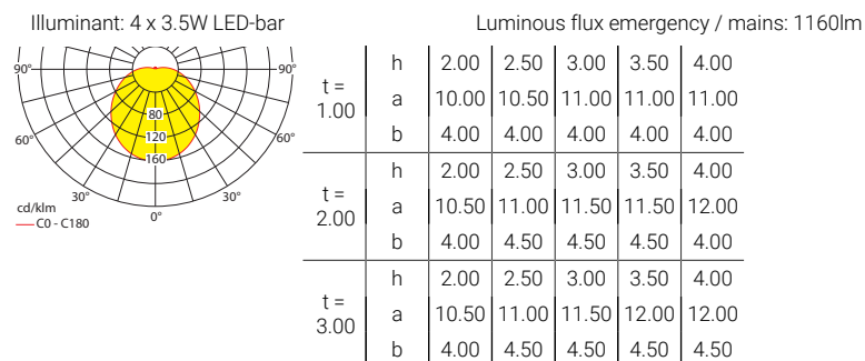
Wall mounting
