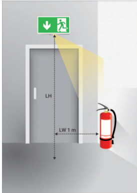
Wandmontage
